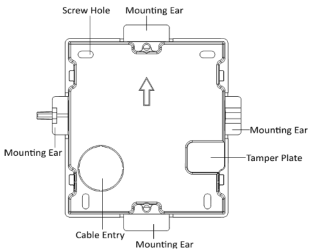
Figure 3-8 Gang Box
