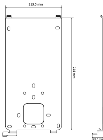
Figure 4-2 Mounting Plate
