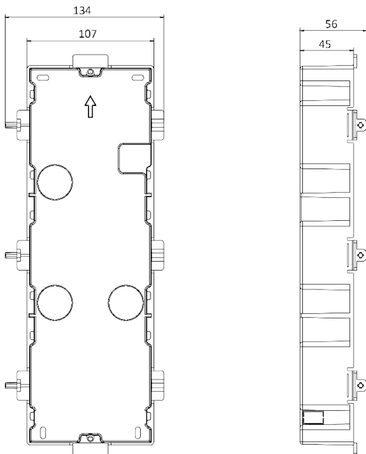
Figure 3-53 Gang Box
