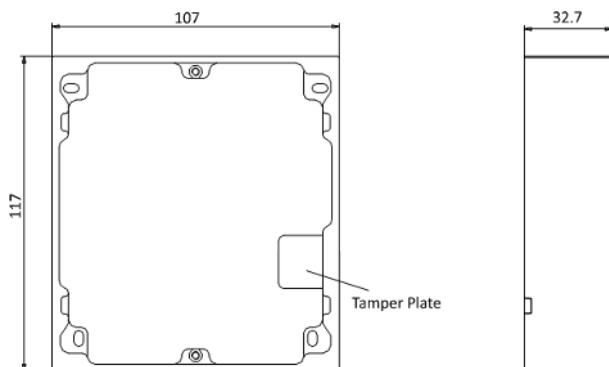
Figure 3-2 Mounting Frame
