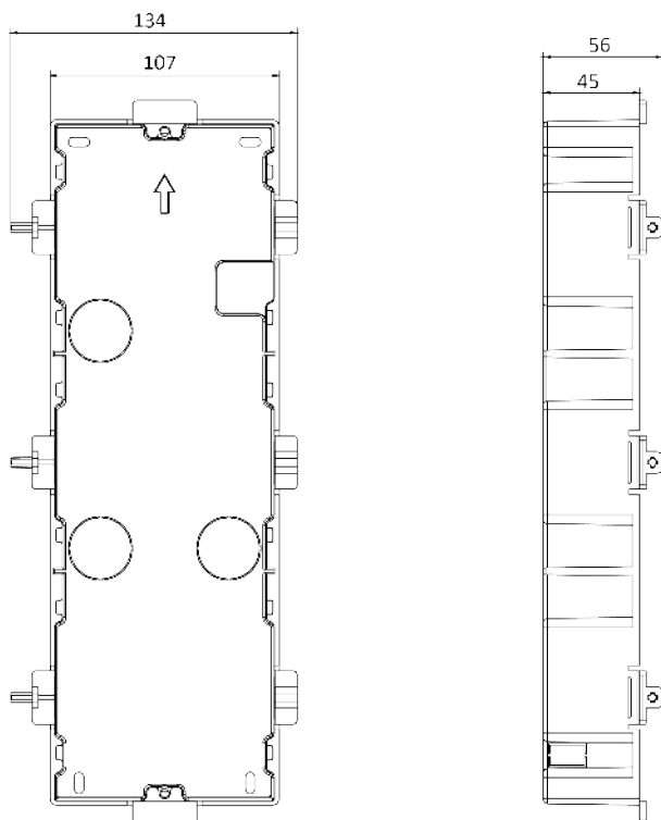
Figure 3-37 Gang Box
