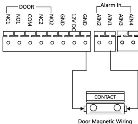
Figure 2-6 Door Contact Wiring
