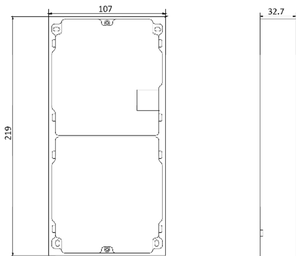
Figure 3-15 Mounting Frame
