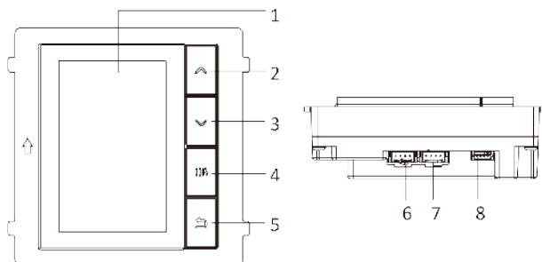
Figure 1-7 Display Module
