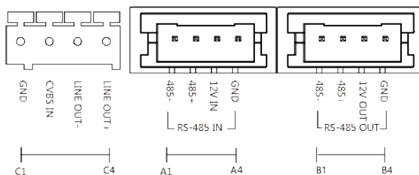
Figure 2-4 Touch-Display Module
