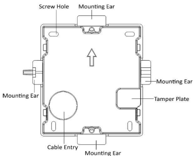
Figure 3-8 Gang Box
